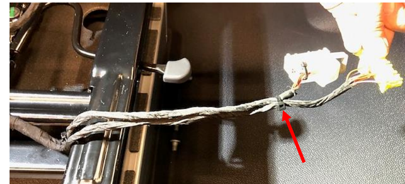
Position the seat harness to the side of the swivel seat frame as shown above and secure the seat harness with push mount cable tie.
